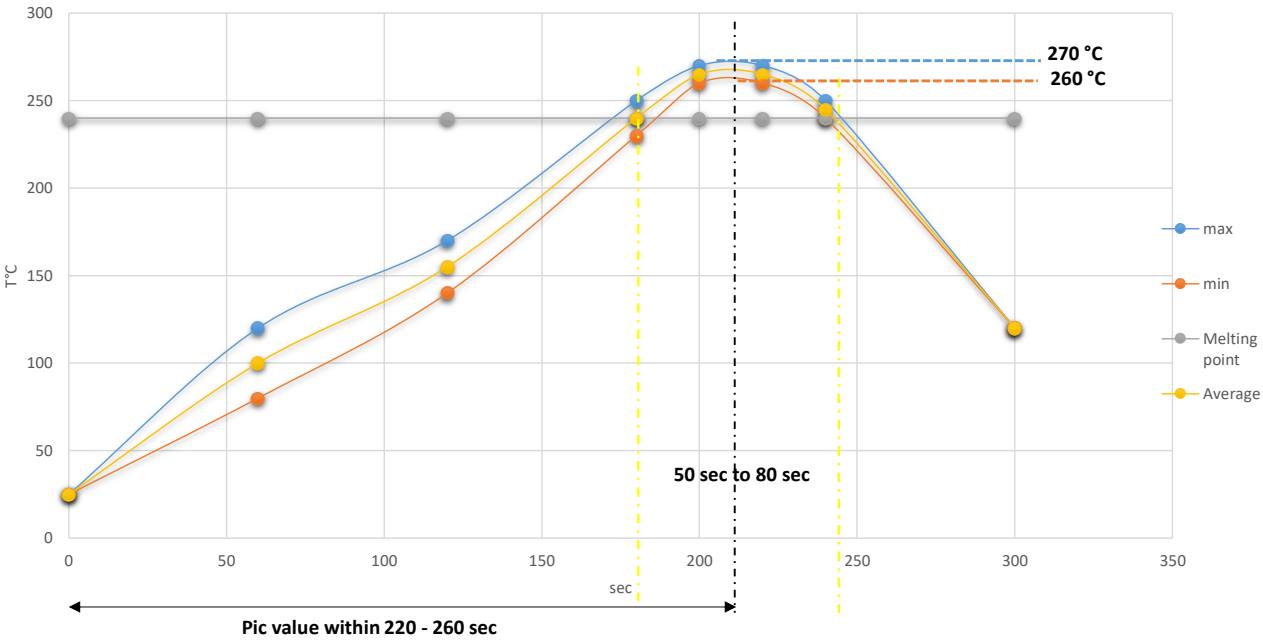
Sn95Sb5 Reflow profile
